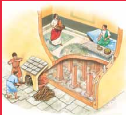
hypocaust
